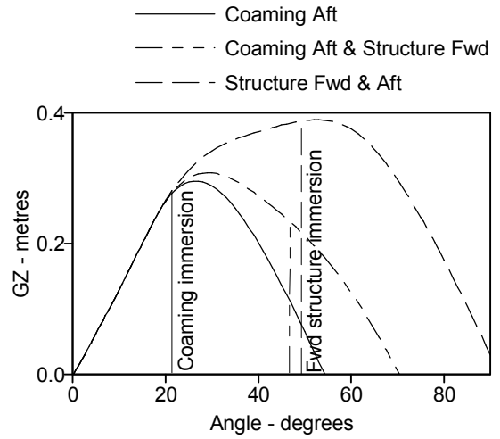
Fig. 4. Stability of the Marchioness model
