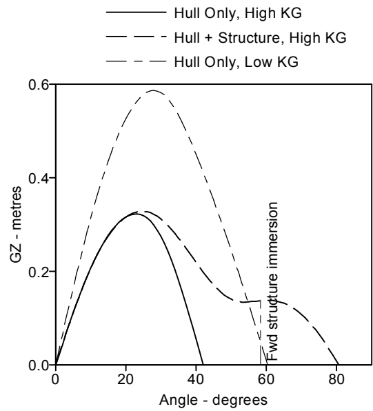
Fig. 5. Stability of the wider vessel model
