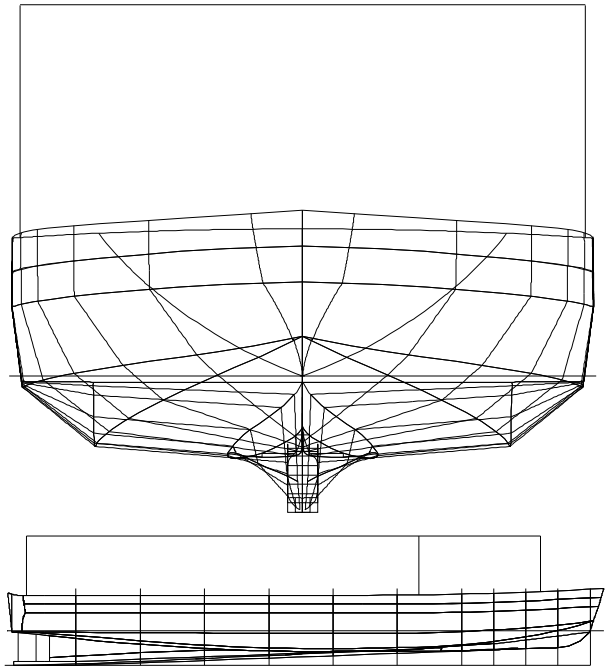
Fig. 2. Wider vessel model
