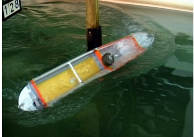
Figure 14. Marchioness, with full superstructure, 5.5 knots, 6.4 seconds after impact
