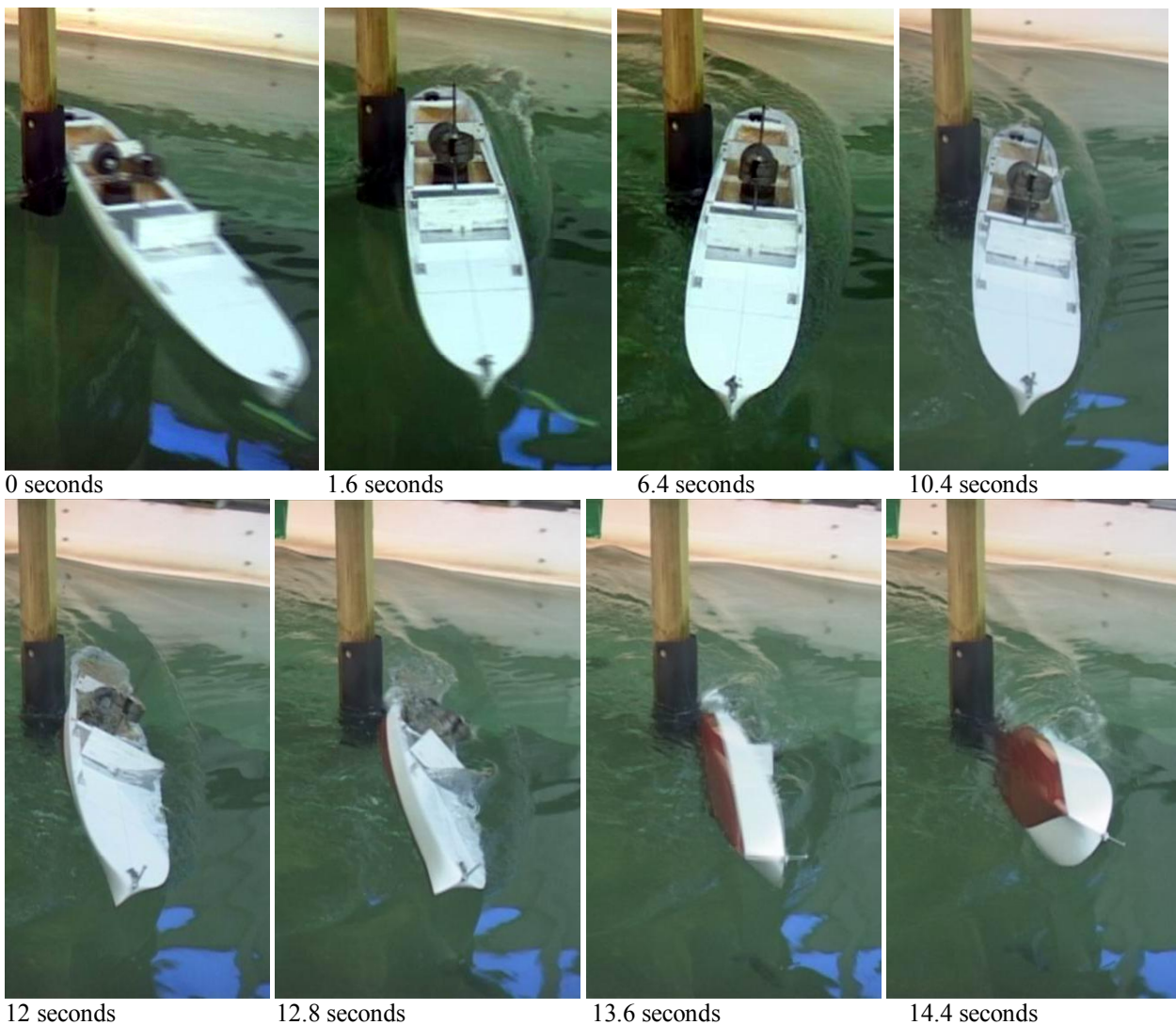
Fig. 12. Simulation of the Marchioness incident. Collision speed 4.5 knots
