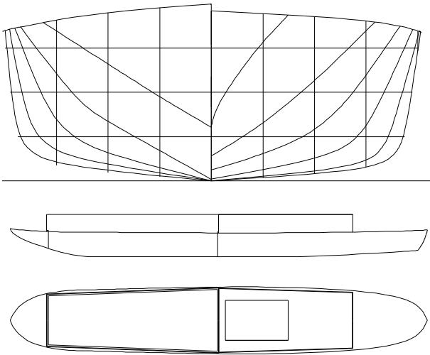
Fig. 1. Marchioness model
