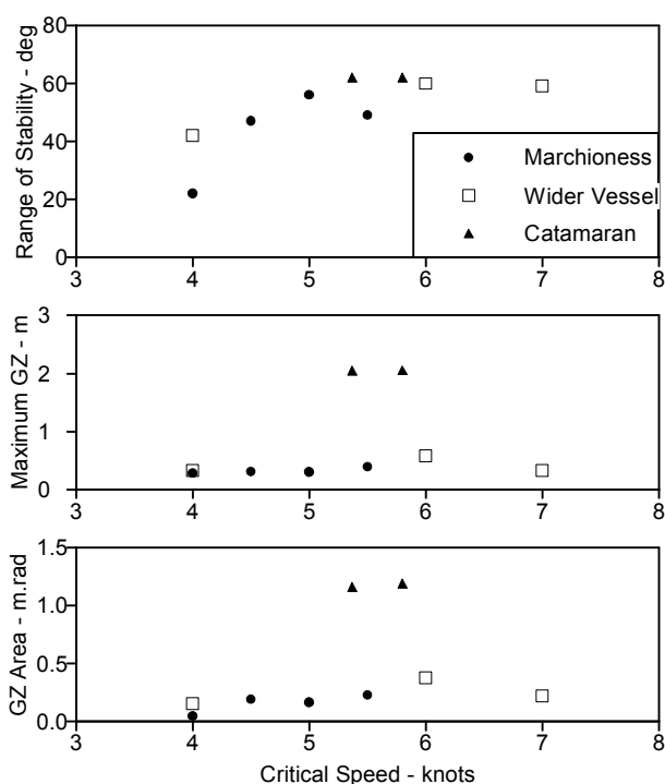
Fig. 10. Variation of critical speed with stability
