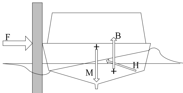
Fig. 9. Forces acting during the quasi-static phase
