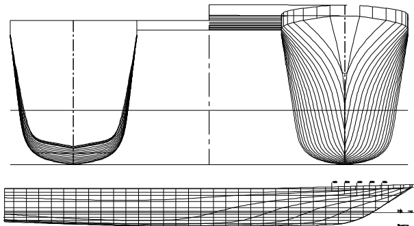
Fig. 3. Catamaran model
