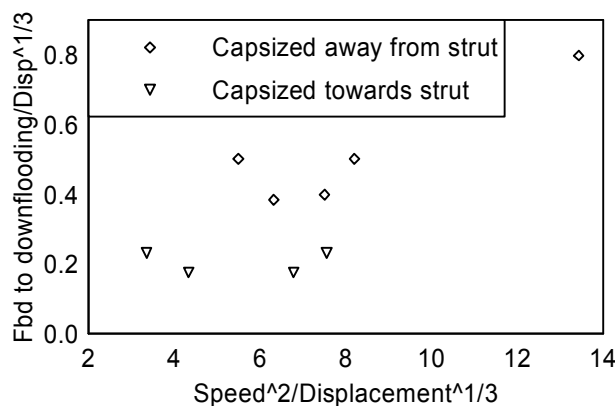
Fig. 11. Variation of critical speed with freeboard
