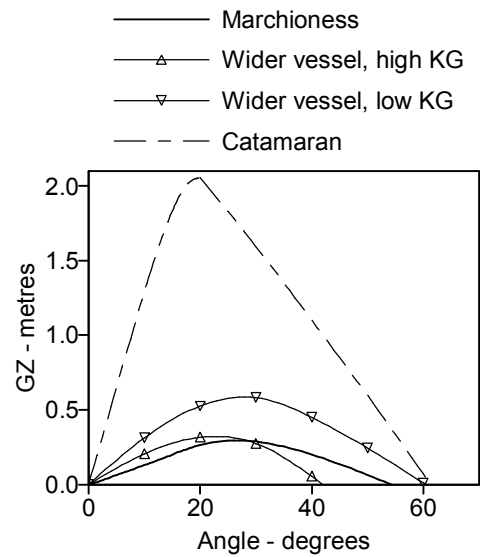
Fig. 6. Comparison of the stability of the three models without superstructures
